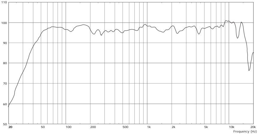
— QM700 - Frequency Response - 2.83V/1m
