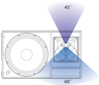
QM700 Horizontal Configuration (front)
