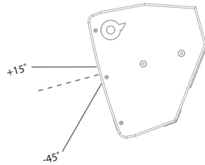
QM700 Horizontal Configuration (side)
